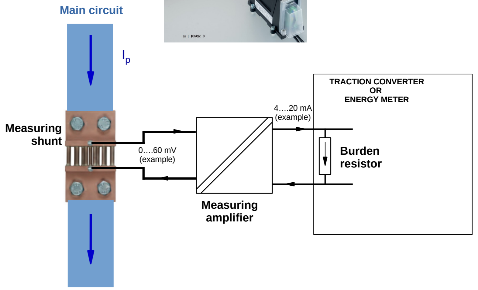
MEASURING SHUNT
