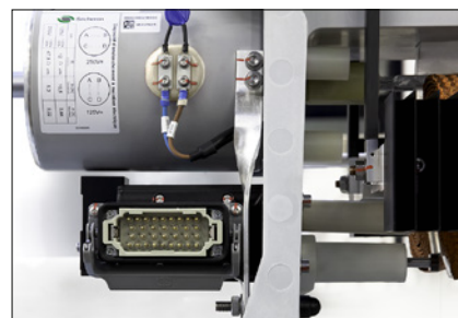
Harting type HAN® 32 EE (Standard)
